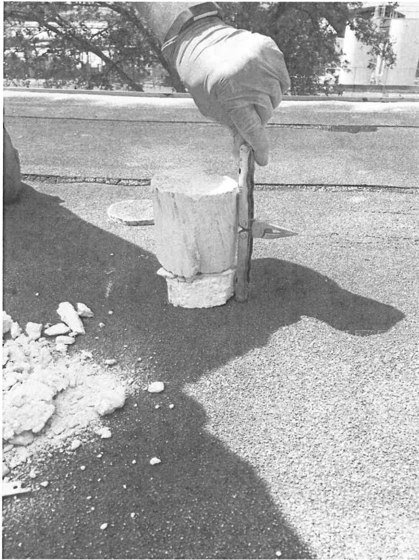
Photo 2: 6" core (2" foam and 4" fire clay) Original roof center of building. Core from Southwest side. 10,920 sq feet.
